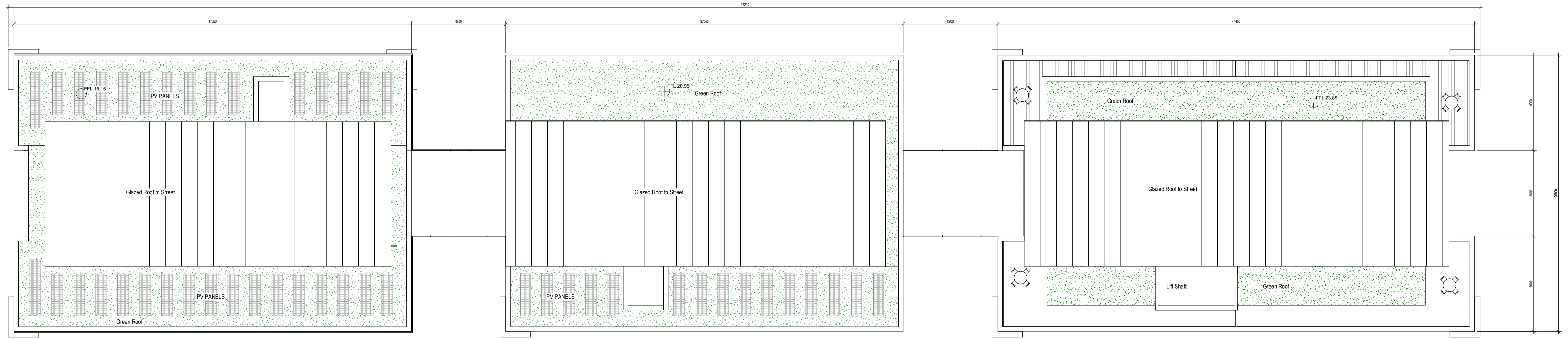
1 Block 01 - Roof Plan 1 : 200 PV Panel Size : 1300mm x 1300mm
